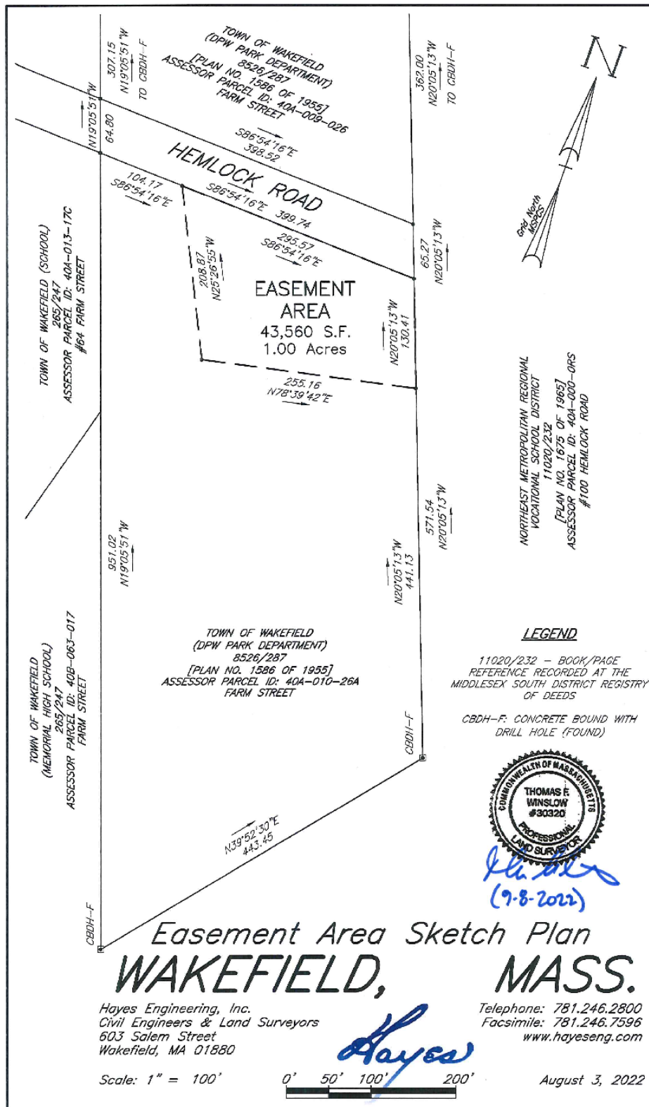
Appendix 3 – Hemlock Road Energy Park Easement Plan
