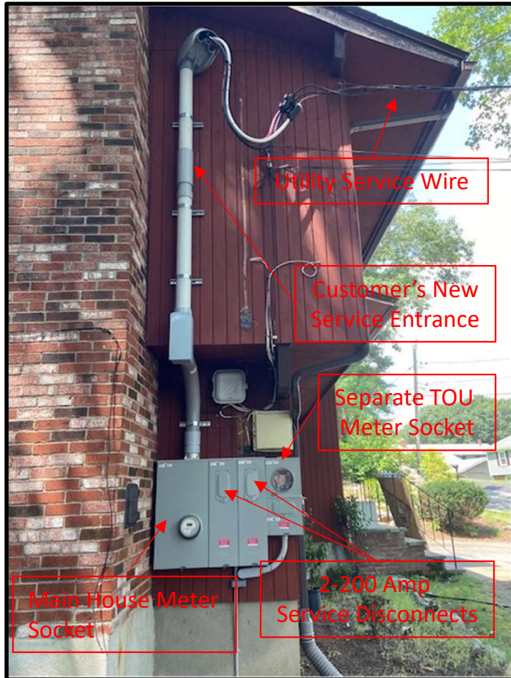
Example of Electric Service And Metering Upgrade
